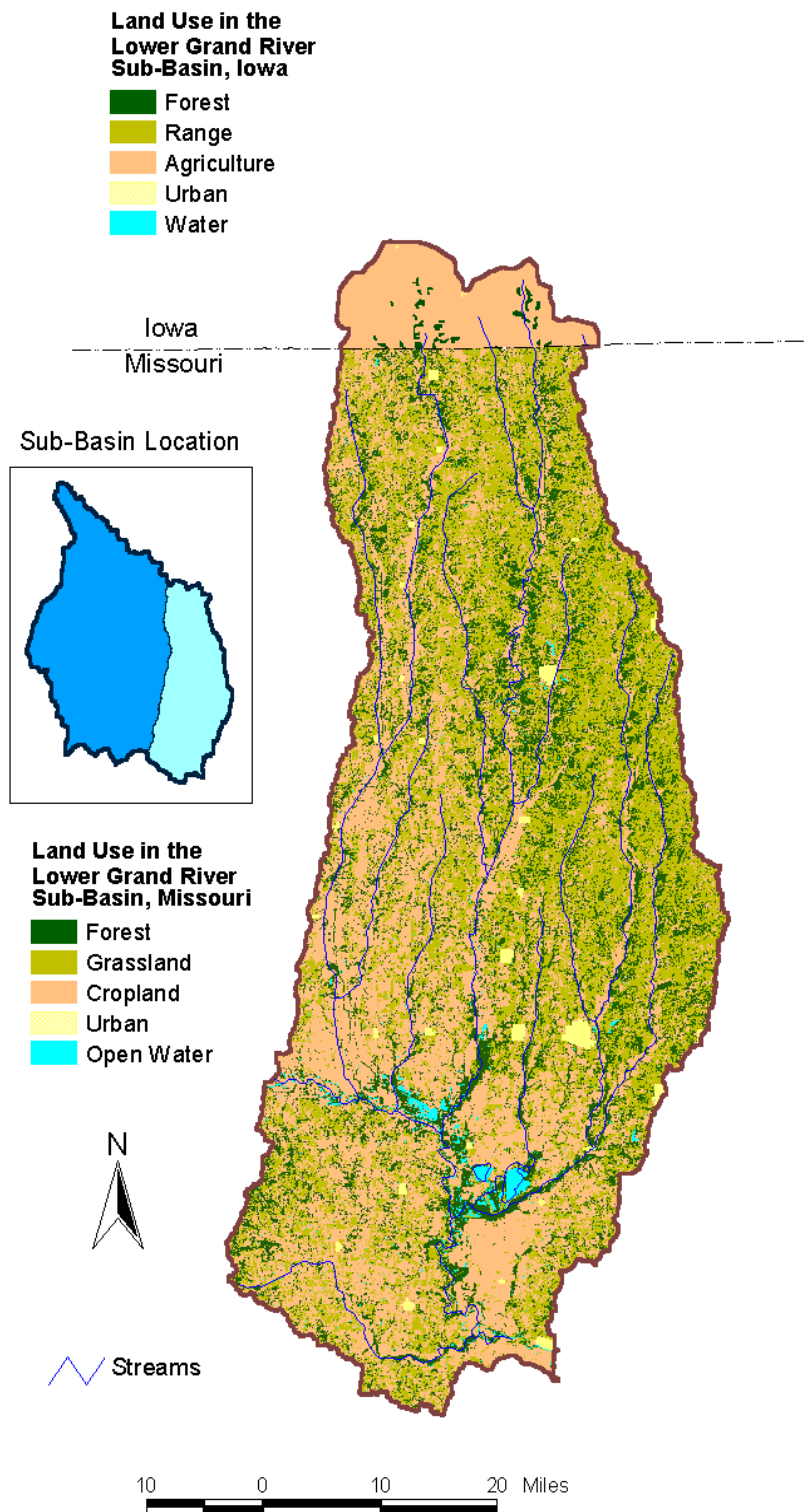
Figure 4a. Land use in the lower Grand River sub-basin in Missouri and Iowa (MORAP 1999, preliminary data).
